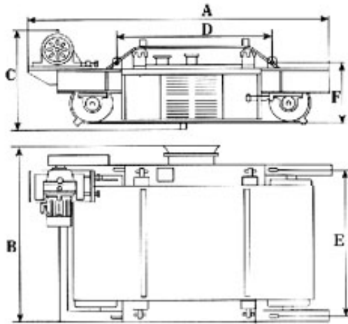
YXDC Self-cleaning Electromagnetic Separators
